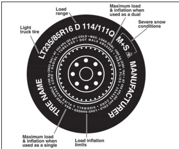
Figure 4: Typical Light Truck Tire Markings
