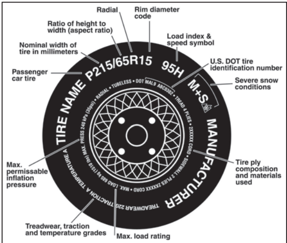
Figure 3: Typical Passenger Tire Markings
